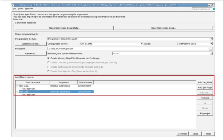
Figure 146. HEX to POF file Conversion Settings for Dual Images Configuration Mode
