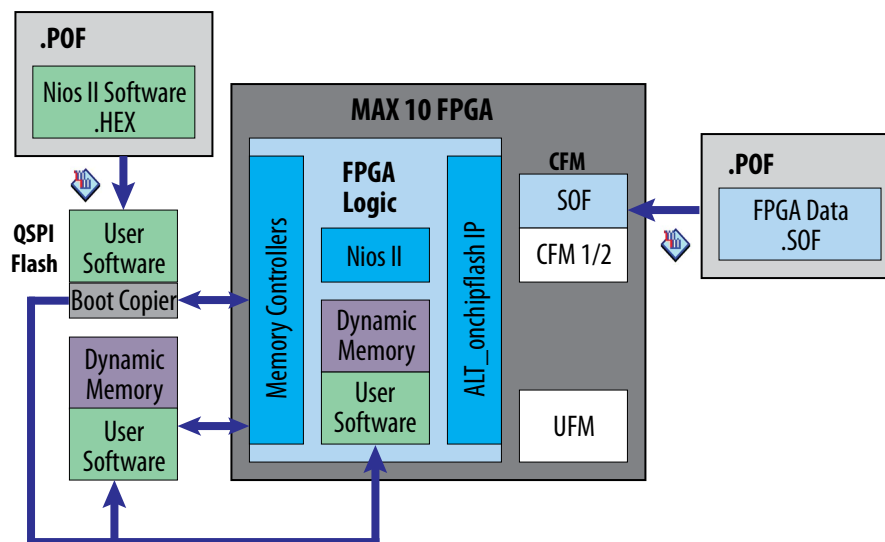
Figure 131. Block Diagram
