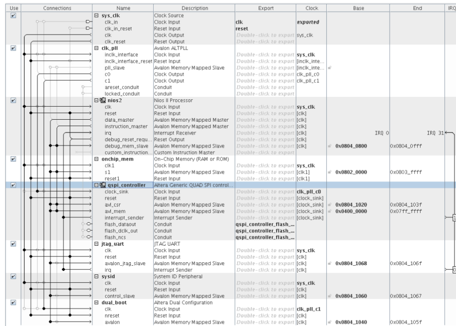
Figure 132. Connection for Generic Quad SPI Controller IP
