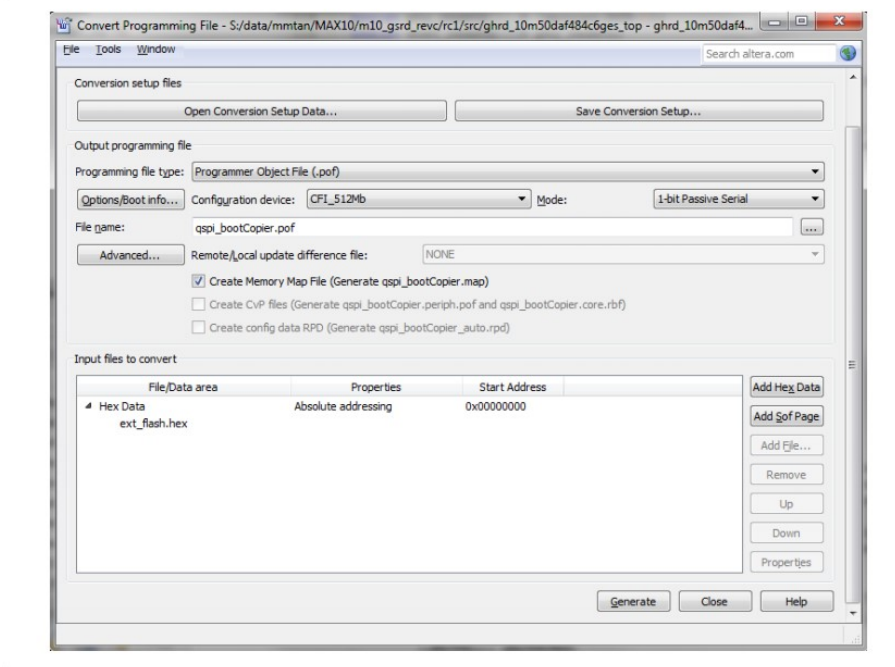
Figure 146. HEX to POF file Conversion Settings for Dual Images Configuration Mode
